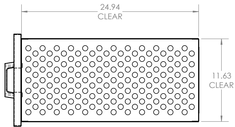
TYPICAL DRAWER
